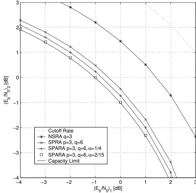
Figure 8: Attainable channel regions for the rate one-third uniformly interleaved accumulate-based ensembles with puncturing depicted in Fig. 5. These regions refer to the asymptotic case where we let N tend to infinity. The communication takes place over J = 2 parallel binary-input AWGN channels, and the bits are equally likely to be assigned over one of these channels ( \alpha_1 = \alpha_2 = \frac{1}{2} ). The achievable channel region refers to optimal ML decoding. The boundaries of these regions are calculated via the generalization of the 1961 Gallager bound followed by the optimization of the tilting measures (see Section 4). The capacity limit and the attainable channel regions which corresponds to the cutoff rate are given as a reference.
