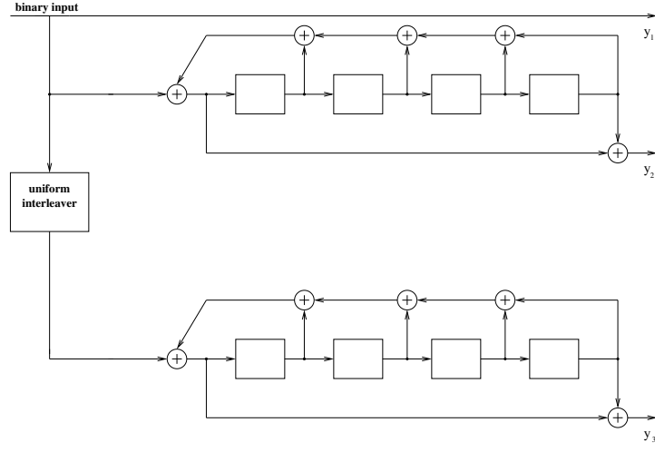
(a) Ensemble of uniformly interleaved turbo codes.
