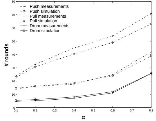
(b) x = 128 .
