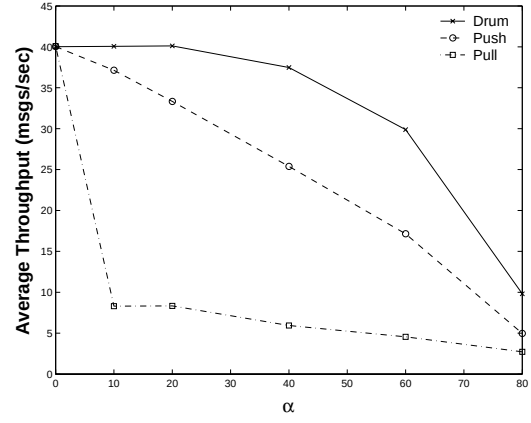
(b) x = 128 .
