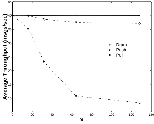
(a) \alpha = 10\% .
