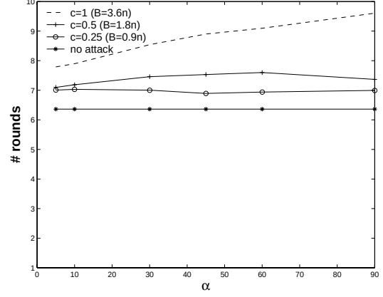
(b) n = 500 .
